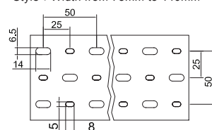
150宽为5排底孔 150 width with 5 lines holes
